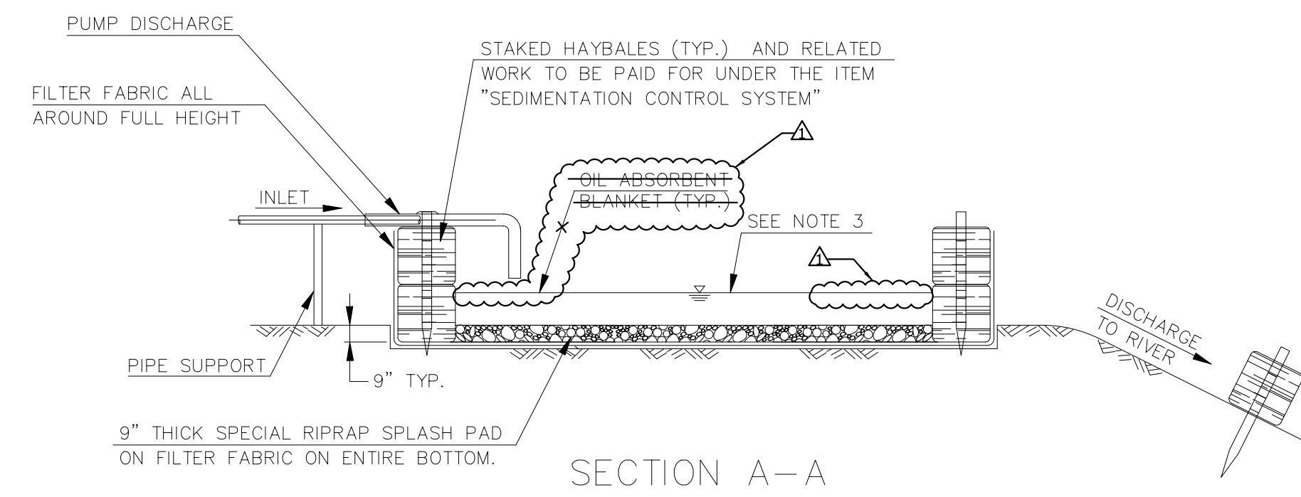
TEMPORARY SEDIMENT BASIN FOR DEWATERING DISCHARGE NOT TO SCALE
